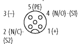
M12-Females 5-pole
