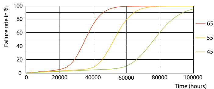
MAS-LEDtube-UE-T8-20240408-75K-FailureRate-LED
