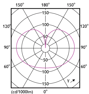
Light Distribution Diagram - LED cła 120W G120 E27 WW FR ND RFSRT4
