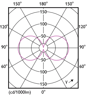
Light Distribution Diagram - MAS LED SON-T UE M 4Klm 19W 740 E27
