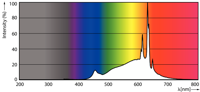
Spectral Power Distribution Colour - MAS LEDBulbDT3.4 -40W E27 CRI95 A60 FR G
