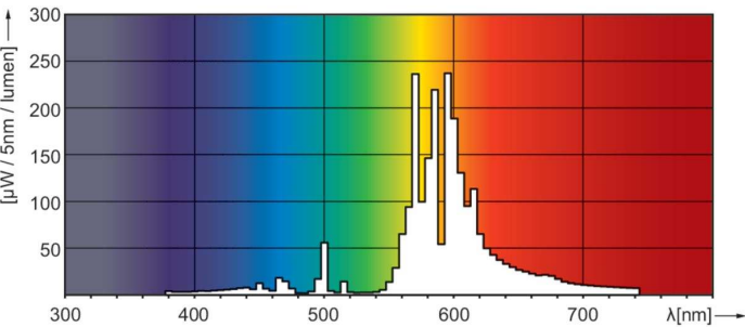
Spectral Power Distribution Colour - MST SON-T PIA Plus 400W E E40 1SL/12
