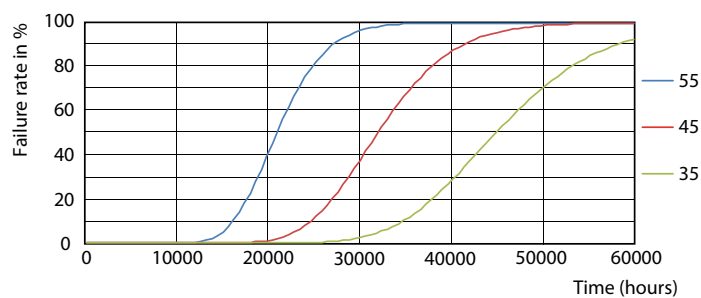
LEDtube COR 1 14,5W 30K FailureRate-LED
