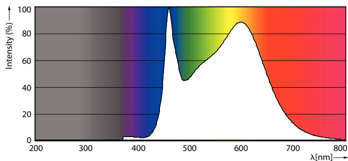
Spectral Power Distribution Colour - CorePro LEDBulb7-60W E27 A60 840
