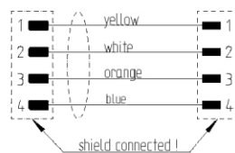
Contact Configuration
