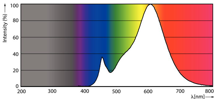
Spectral Power Distribution Colour - LEDbulb ND 10-75W A60 E27 827 1CT
