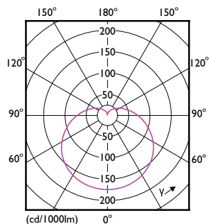
Light Distribution Diagram - LEDbulb ND 10-75W A60 E27 827 1CT
