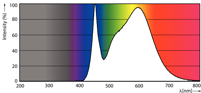
Spectral Power Distribution Colour - LEDbulb ND 4.9-40W A60 E27 840 1CT
