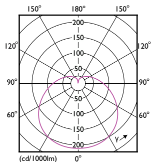
Light Distribution Diagram - LEDbulb ND 4.9-40W A60 E27 840 1CT
