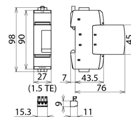
Dimension drawing DG SE CI 440 FM
