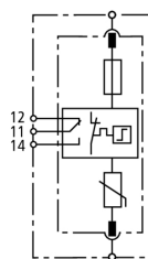
Basic circuit diagram DG SE CI 440 FM
