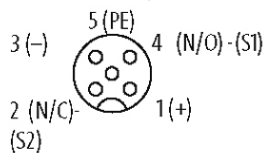
M12-Females 5-pole
