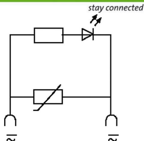
VDR + LED
