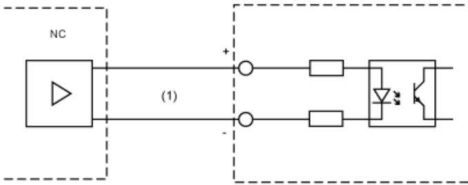
(1) Opto-isolated signals
