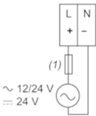
(1) Type T fuse (Controller: 1.25 A , Expansion: 1 A)
