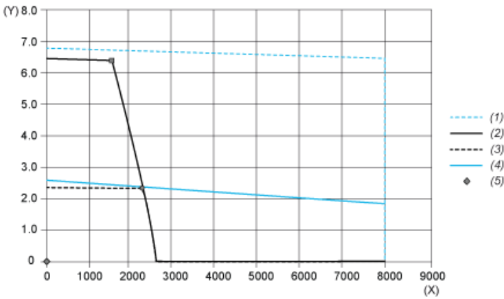
Torque/Speed Curves with 208 V Three Phases Supply Voltage
