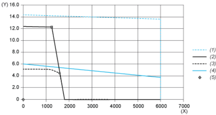
Torque/Speed Curves with 115 V Single Phase Supply Voltage
