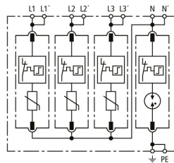
Basic circuit diagram DG MP TT 275
