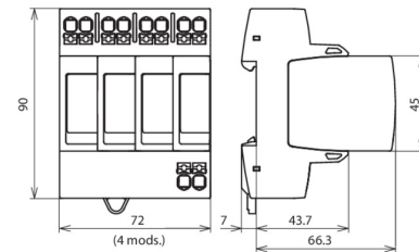
Dimension drawing DG MP TT 275
