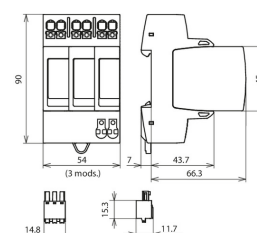
Dimension drawing DG MP YPV 1200 FM
