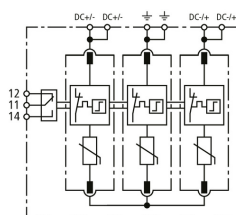
Basic circuit diagram DG MP YPV 1200 FM
