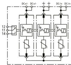
Basic circuit diagram DG MP YPV 1500 FM
