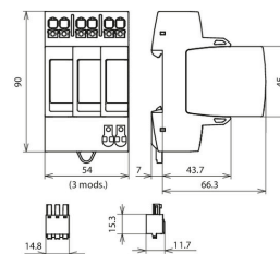
Dimension drawing DG MP YPV 1500 FM
