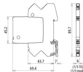
Dimension drawing BCO ML2 BD 12
