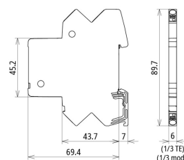
Dimension drawing BCO CL2 BE 24
