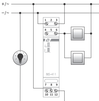
Connection with control pulse +
