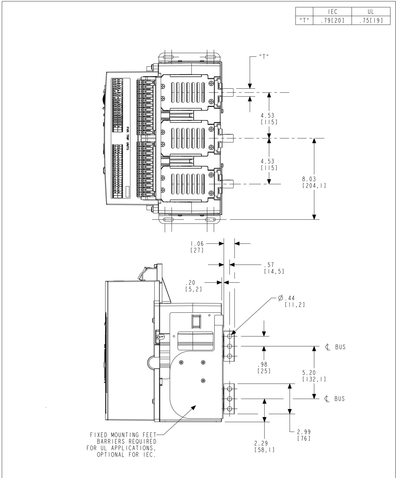
Figure 54. Three-pole fixed breaker - top/side views with centered three-hole vertical bus adapter in inches (mm).
