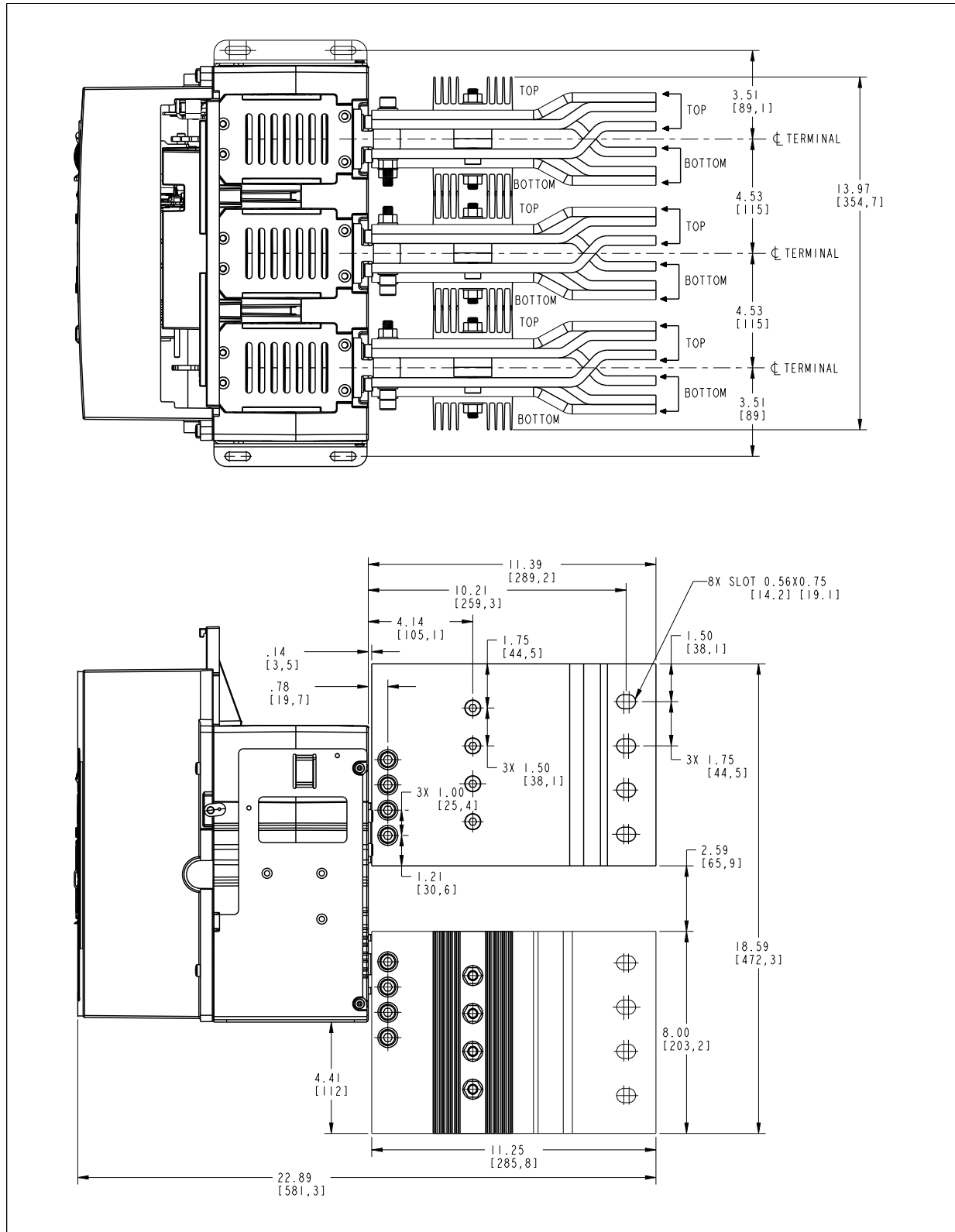
Figure 57. Three-pole fixed breaker-top/side views with stamped adapter in inches (mm)-UL only.
