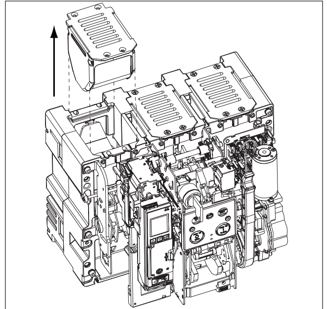
Figure 71. Step 4.
