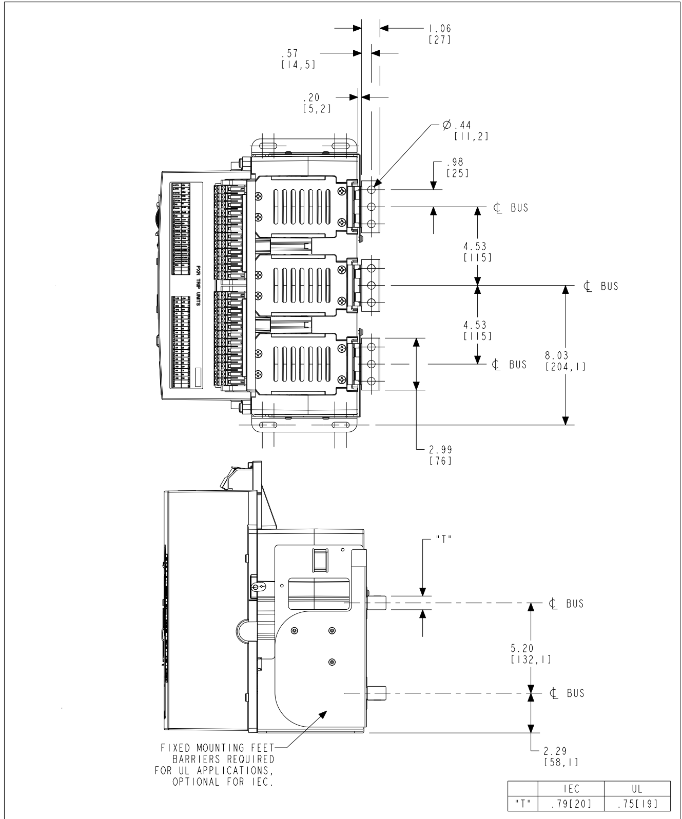
Figure 53. Three-pole fixed breaker - top/side views with centered three-hole horizontal bus adapter in inches (mm).
