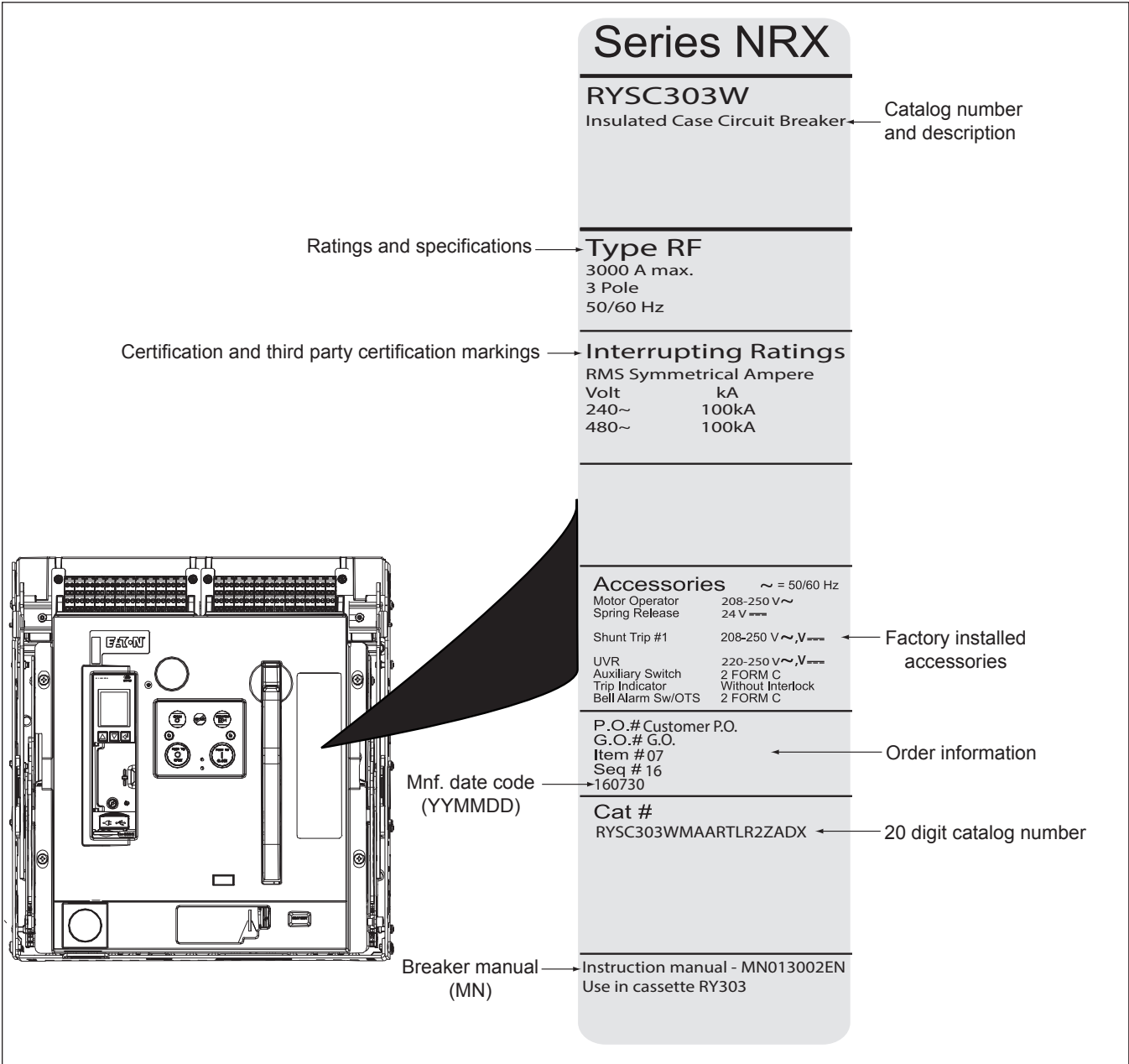
Figure 1. Series NRX nameplate location.
