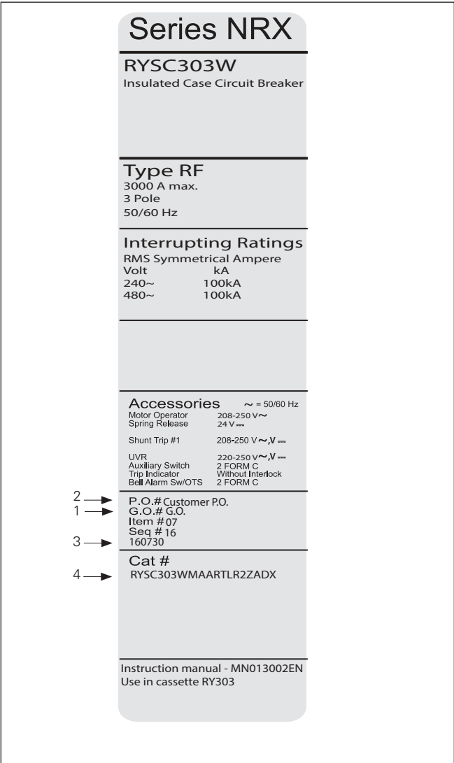
Figure 67. Typical nameplate information.
