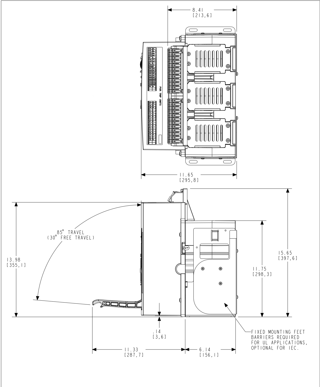
Figure 52. Three-pole fixed breaker - top/side views in inches (mm).
