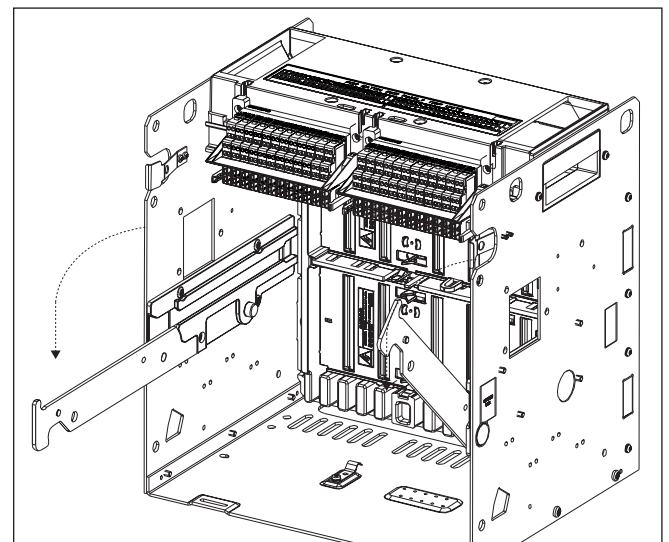
Figure 13. Step 2.
