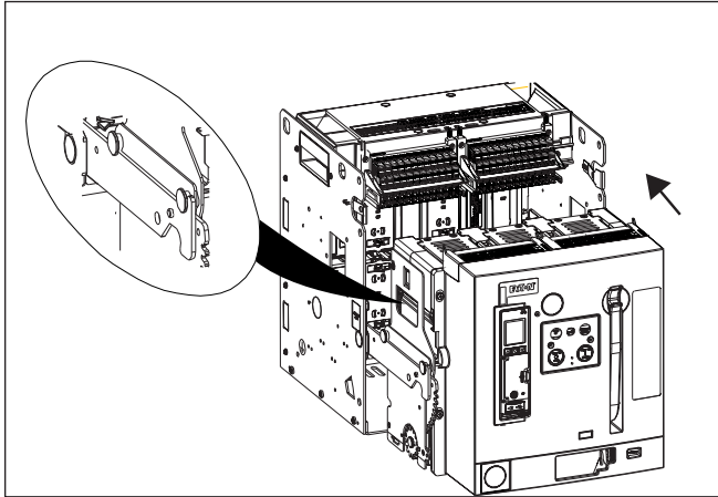
Figure 14. Step 3.
