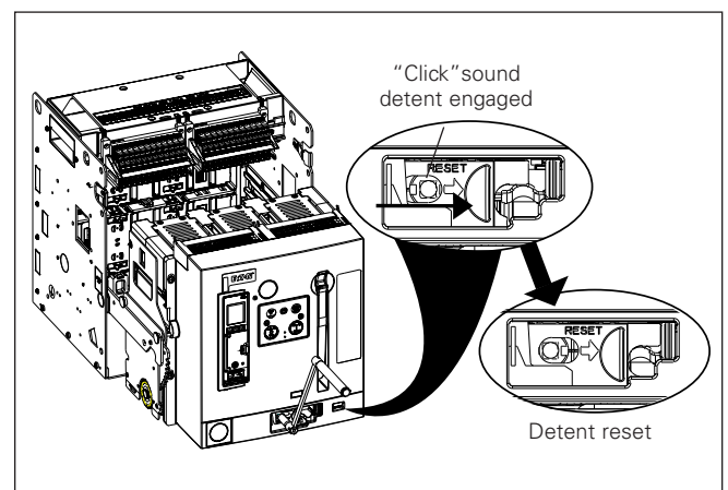
Figure 20a. Step 2.
