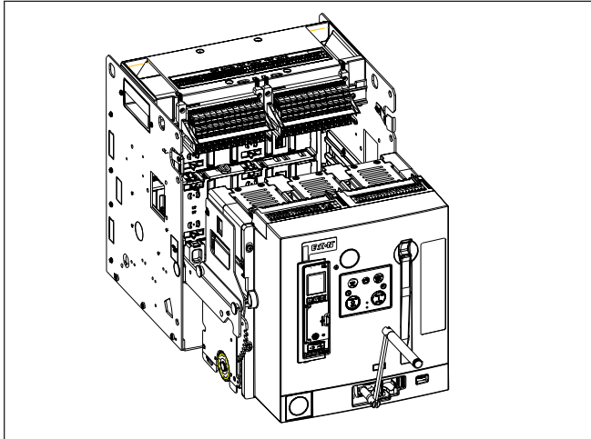
Figure 21. Step 3.
