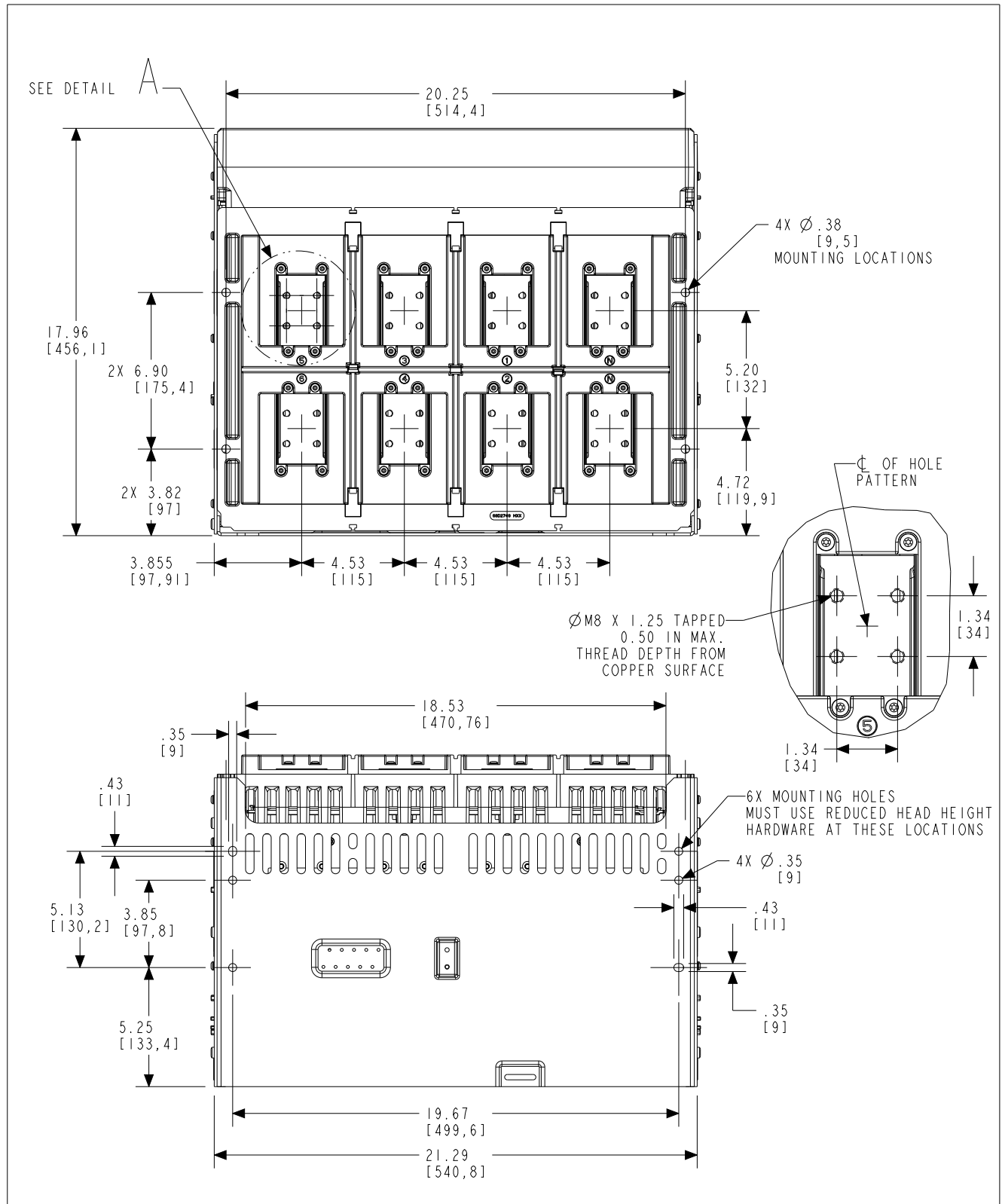
Figure 42. Four-pole drawout cassette - rear/bottom views in inches (mm).
