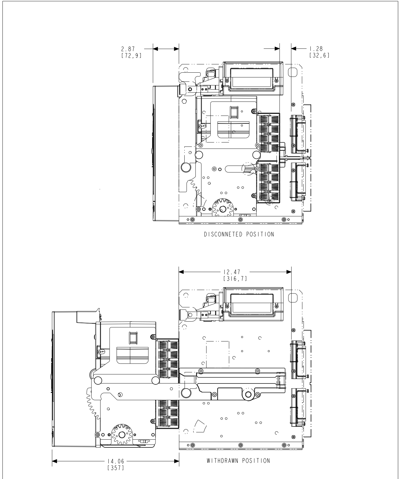
Figure 44. Four-pole drawout cassette - side views DISCONNECTED and WITHDRAWN positions in inches (mm).
