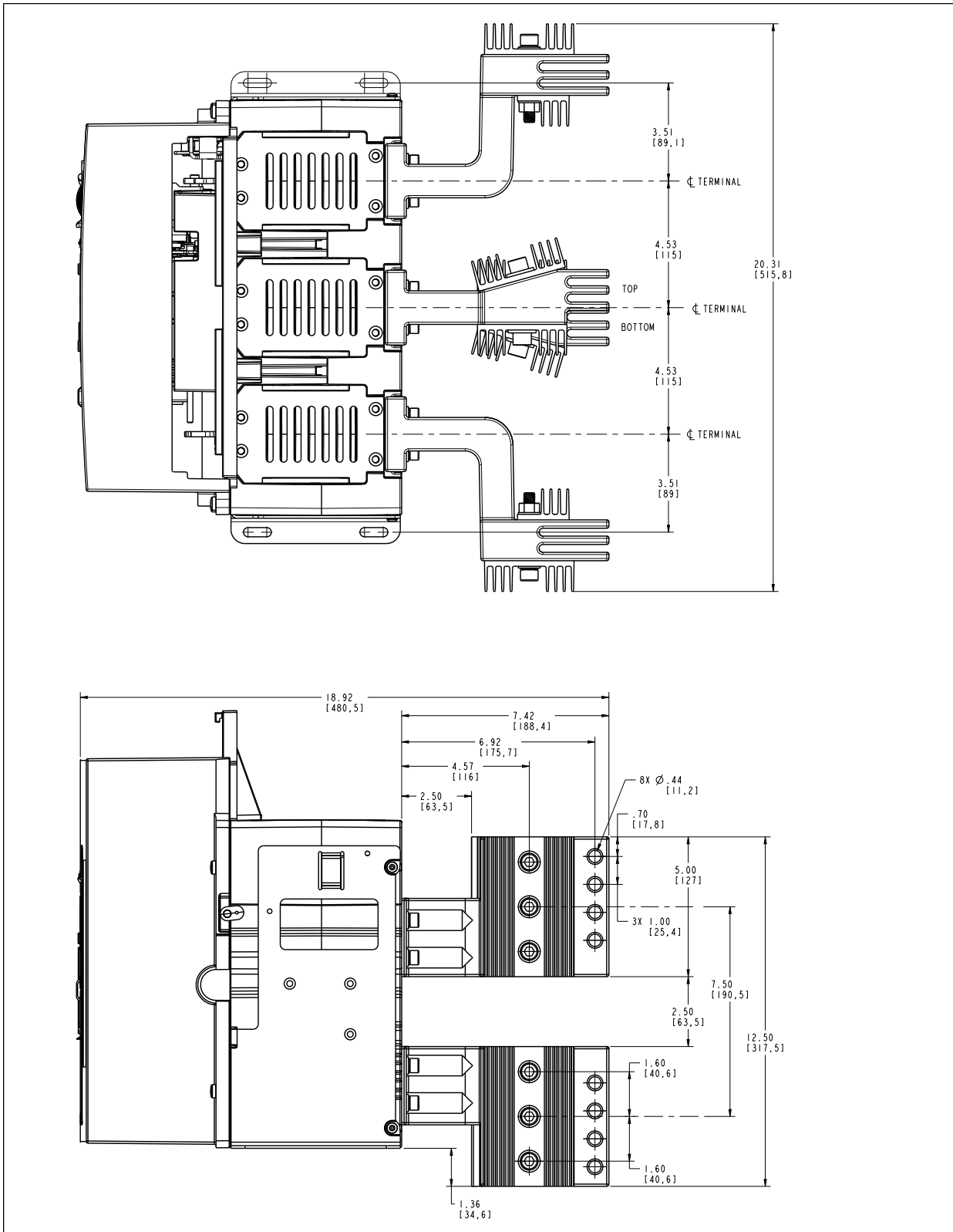
Figure 58. Three-pole fixed breaker-top/side views with casted adapter in inches (mm)-UL only.
