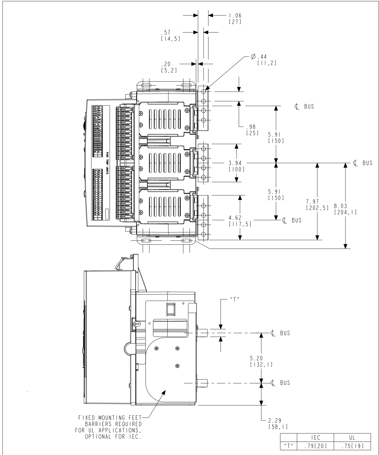
Figure 55. Three-pole fixed breaker - top/side views with offset four-hole horizontal bus adapter in inches (mm).
