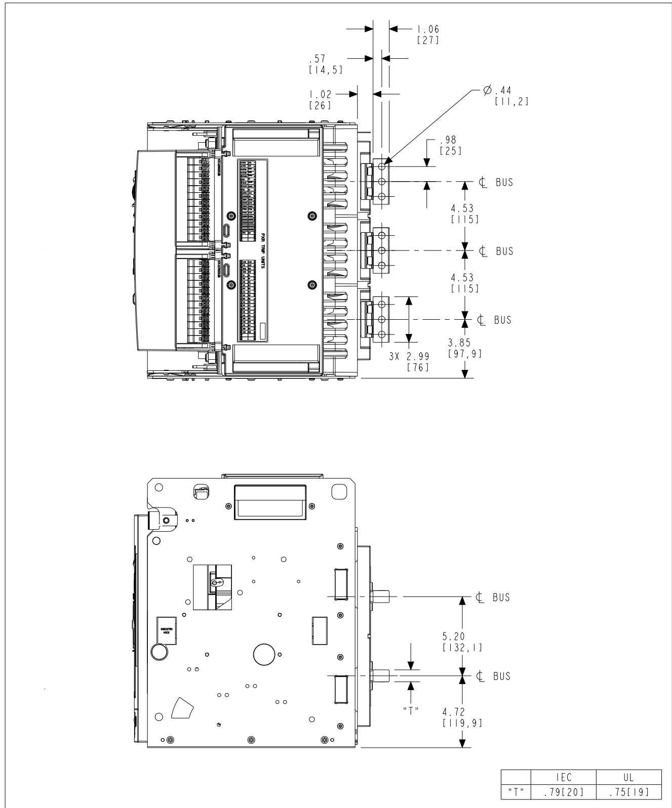
Figure 36. Three-pole drawout cassette - top/side views with centered three-hole horizontal bus adapters in inches (mm).
