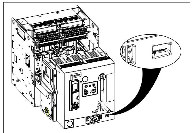
Figure 20. Step 2.
