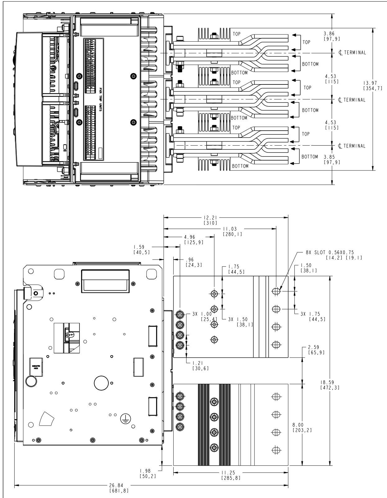
Figure 40. Three-pole drawout cassette-top/side views with stamped adapter in inches (mm)-UL only.
