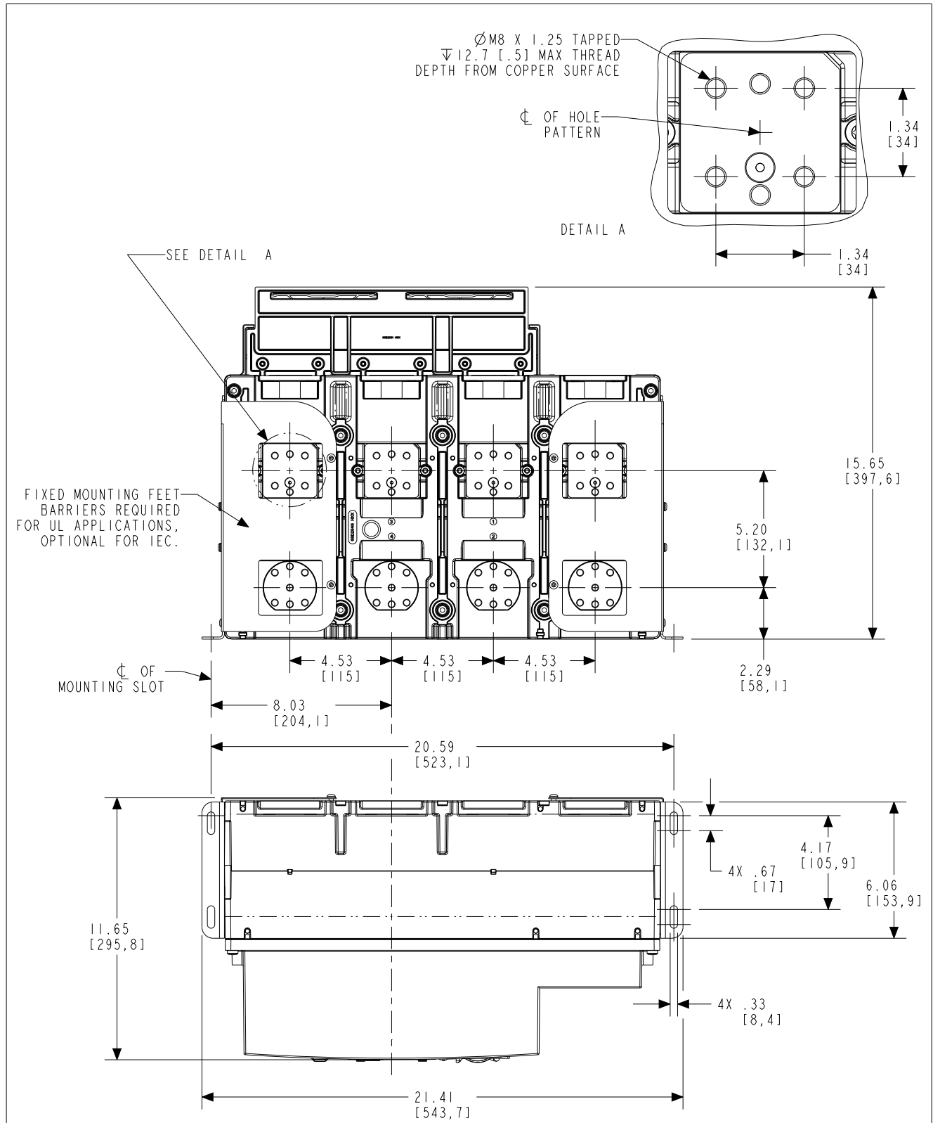
Figure 59. Four-pole fixed breaker - rear/bottom views in inches (mm).
