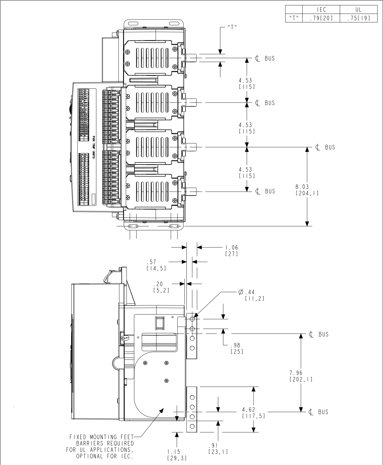
Figure 64. Four-pole fixed breaker - top/side views with offset four-hole vertical bus adapter in inches (mm).
