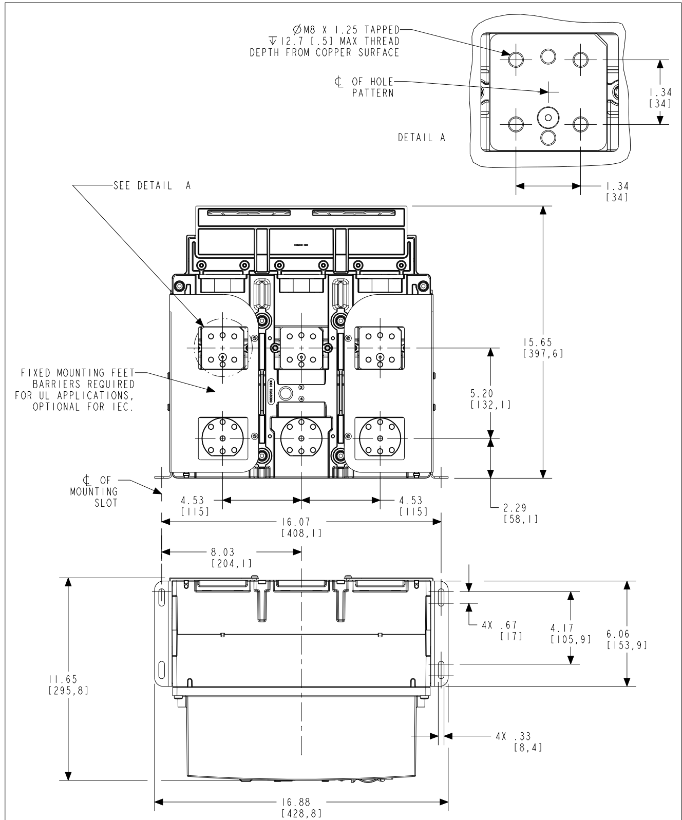
Figure 51. Three-pole fixed breaker - rear/bottom views in inches (mm).
