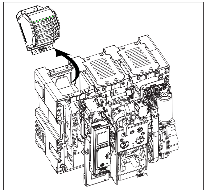
Figure 72. Step 6.
