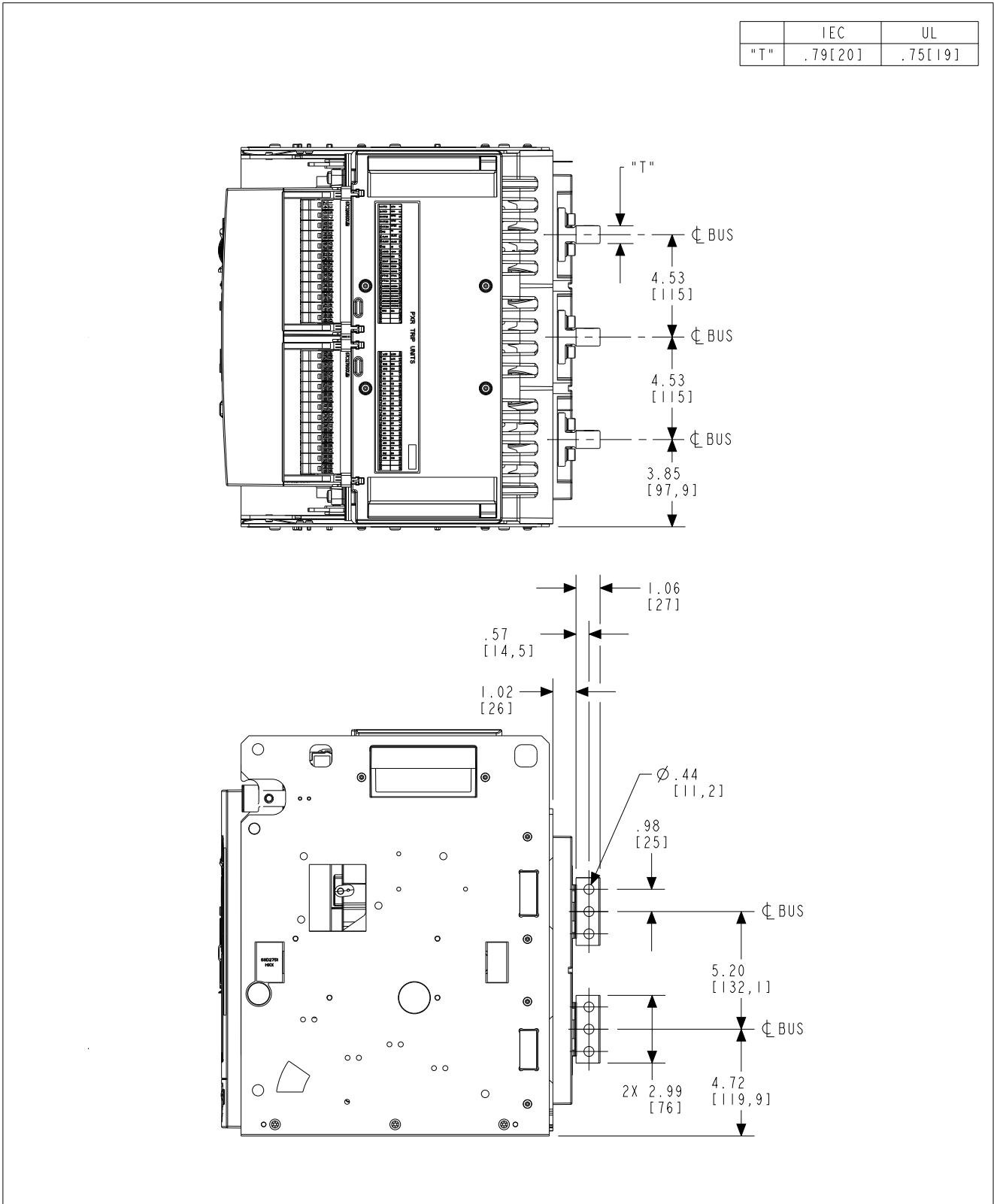
Figure 37. Three-pole drawout cassette - top/side views with centered three-hole vertical bus adapters in inches (mm).
