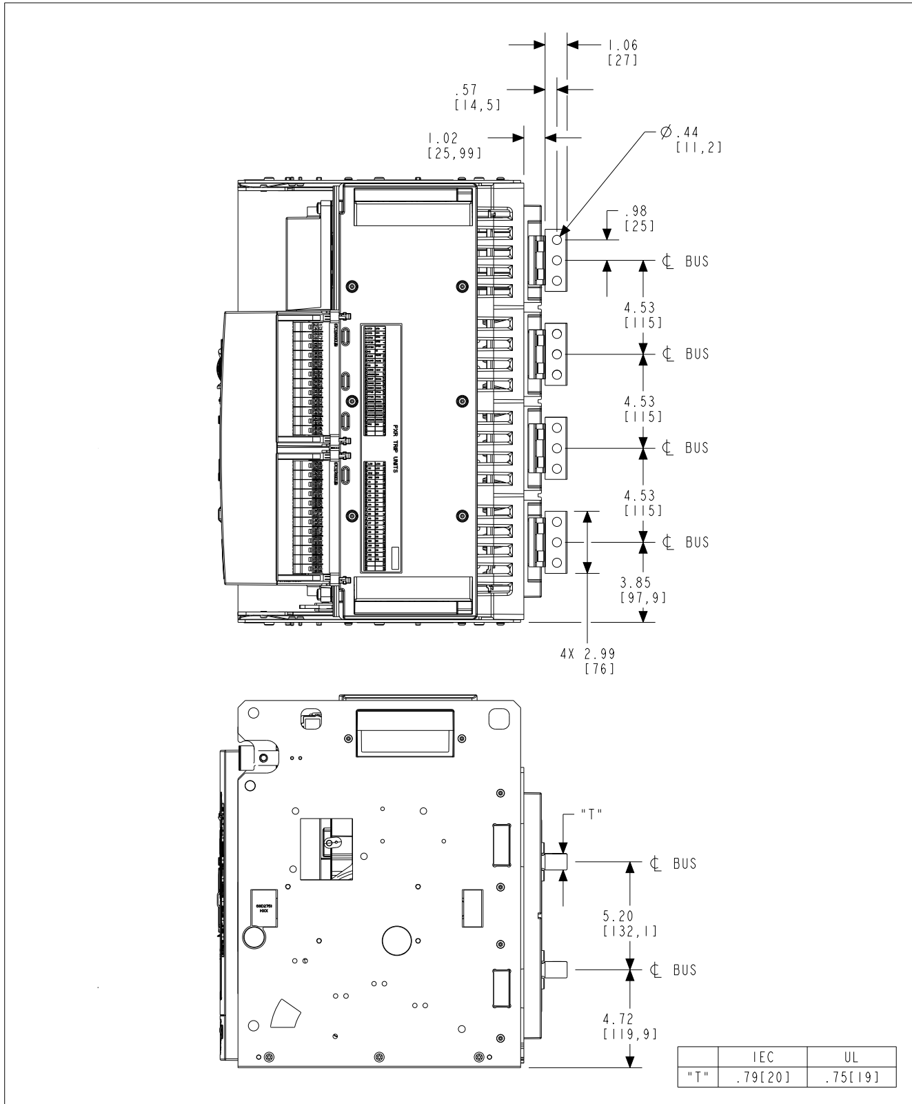
Figure 45. Four-pole drawout cassette - top/side views with centered three-hole horizontal bus adapters in inches (mm).
