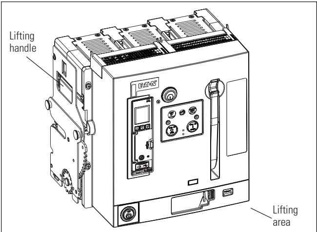
Figure 8. Step 3.
