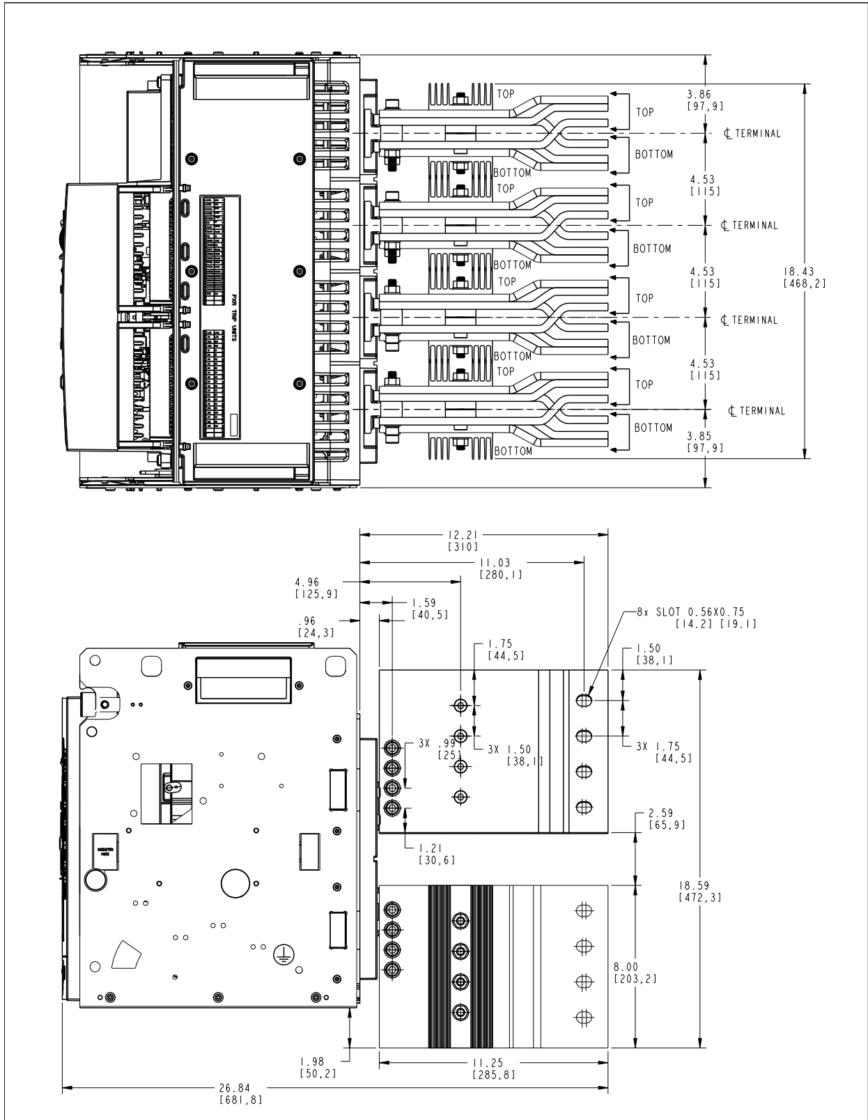
Figure 49. Four-pole drawout cassette-top/side views with stamped adapter in inches (mm)-UL only.
