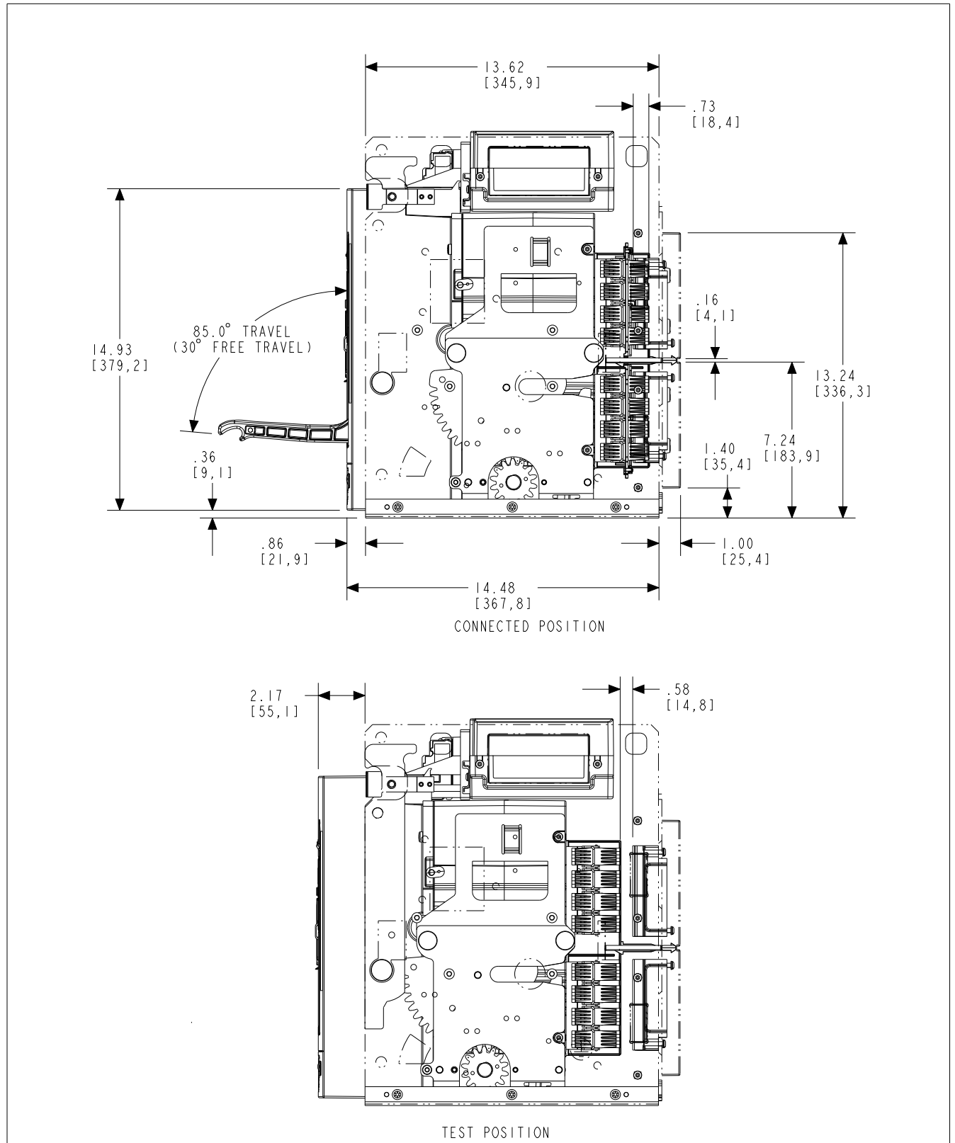
Figure 34. Three-pole drawout cassette - side views CONNECTED and TEST positions in inches (mm).
