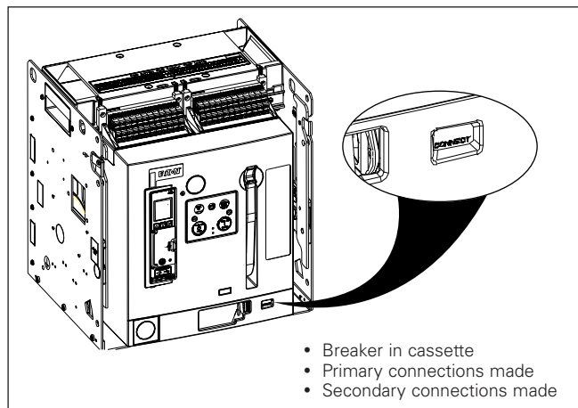
Figure 19. CONNECT position.
