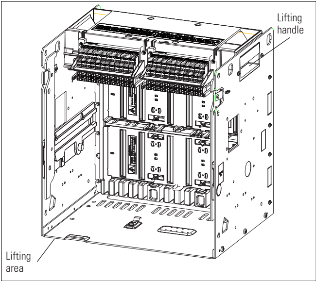
Figure 10. Step 3.
