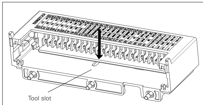
Figure 69. Step 2.
