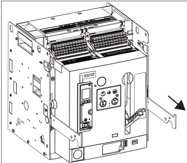
Figure 15. Step 4.
