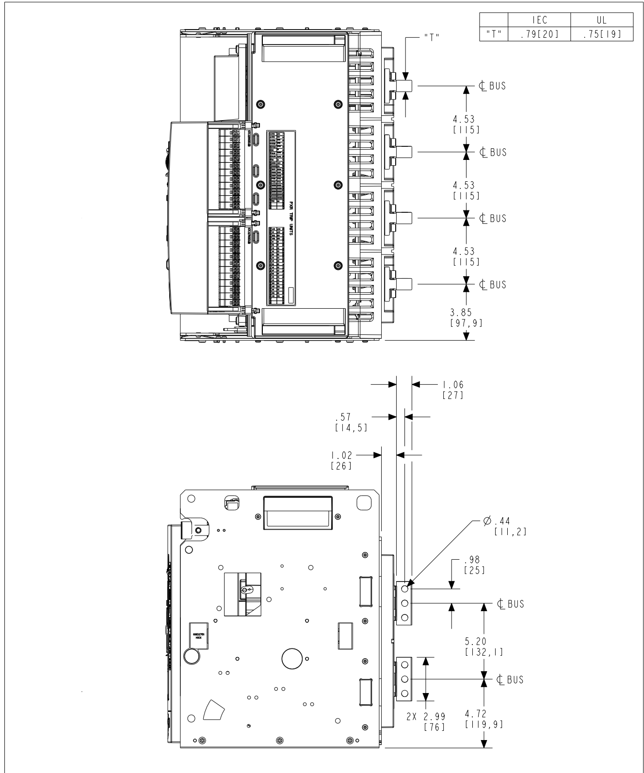
Figure 46. Four-pole drawout cassette-top/side views with centered three-hole vertical bus adapters in inches (mm).
