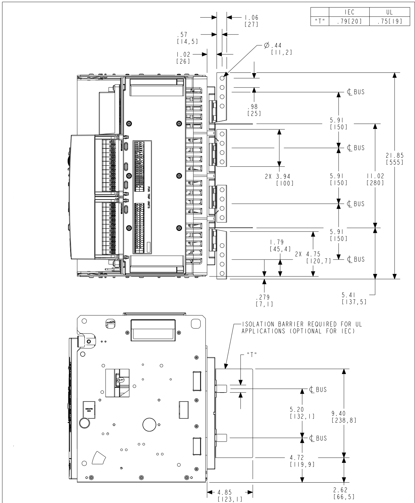
Figure 47. Four-pole drawout cassette- top/side views with offset four-hole horizontal bus adapters in inches (mm).
