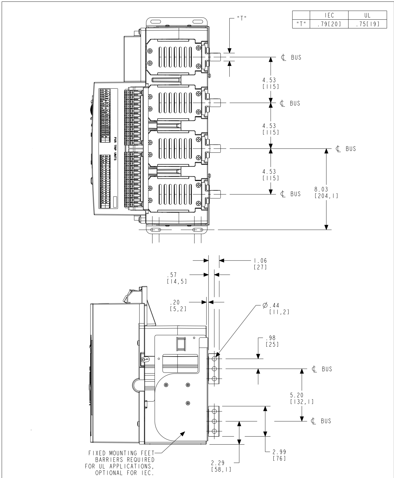
Figure 62. Four-pole fixed breaker - top/side views with centered three-hole vertical bus adapter in inches (mm).
