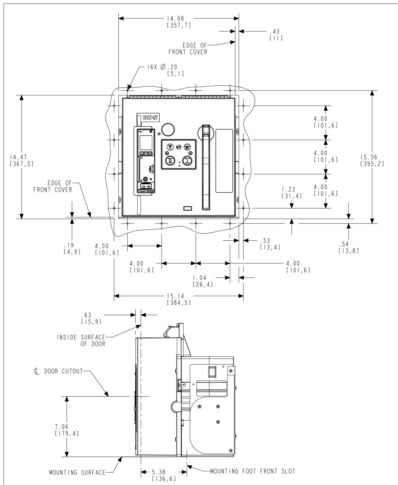
Figure 66. Three-pole/four-pole fixed breaker - front door cutout details in inches (mm).
