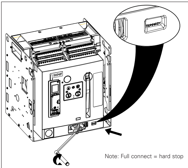
Figure 22. Step 4.
