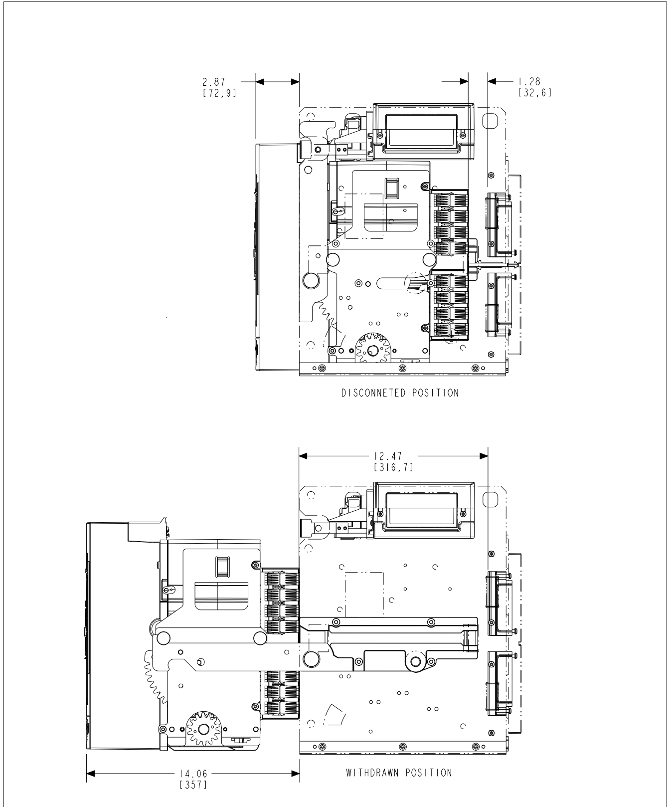
Figure 35. Three-pole drawout cassette - side views DISCONNECTED and WITHDRAWN positions in inches (mm).
