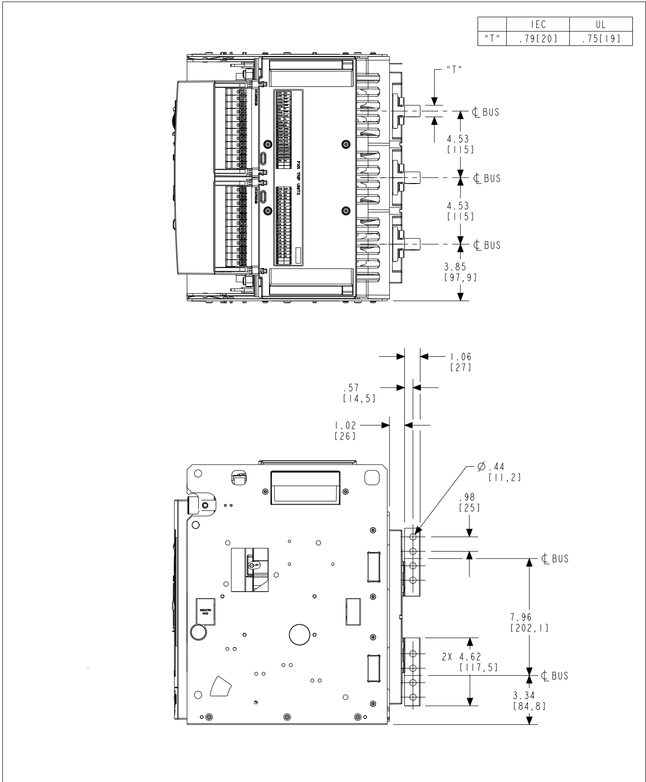
Figure 39. Three-pole drawout cassette - top/side views with offset four-hole vertical bus adapters in inches (mm).
