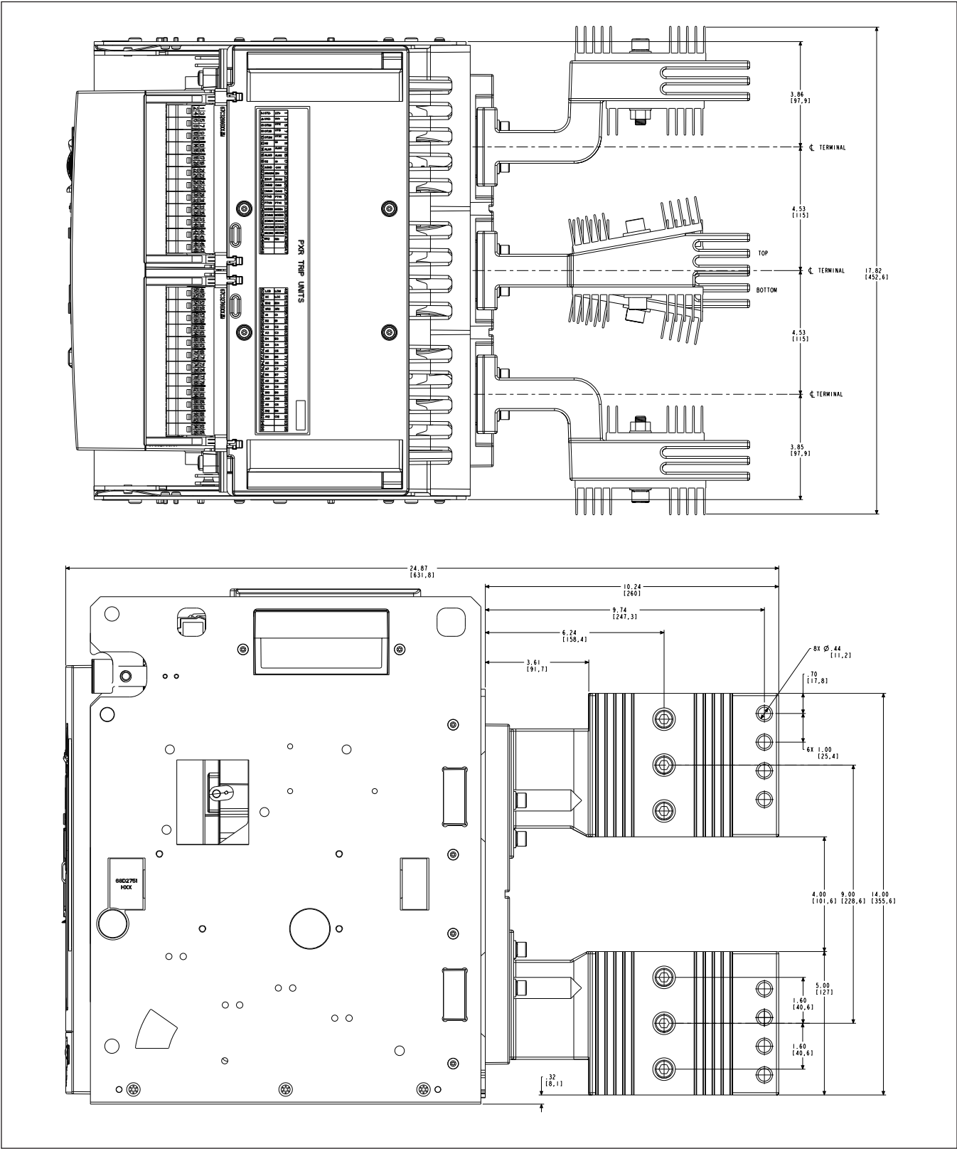
Figure 41. Three-pole drawout cassette-top/side views with casted adapter in inches (mm)-UL only.
