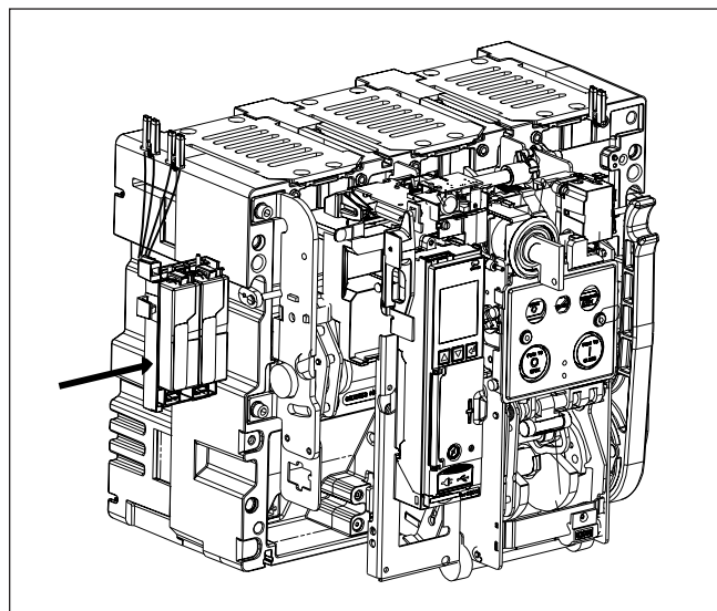
Figure 32. Right accessory tray.
