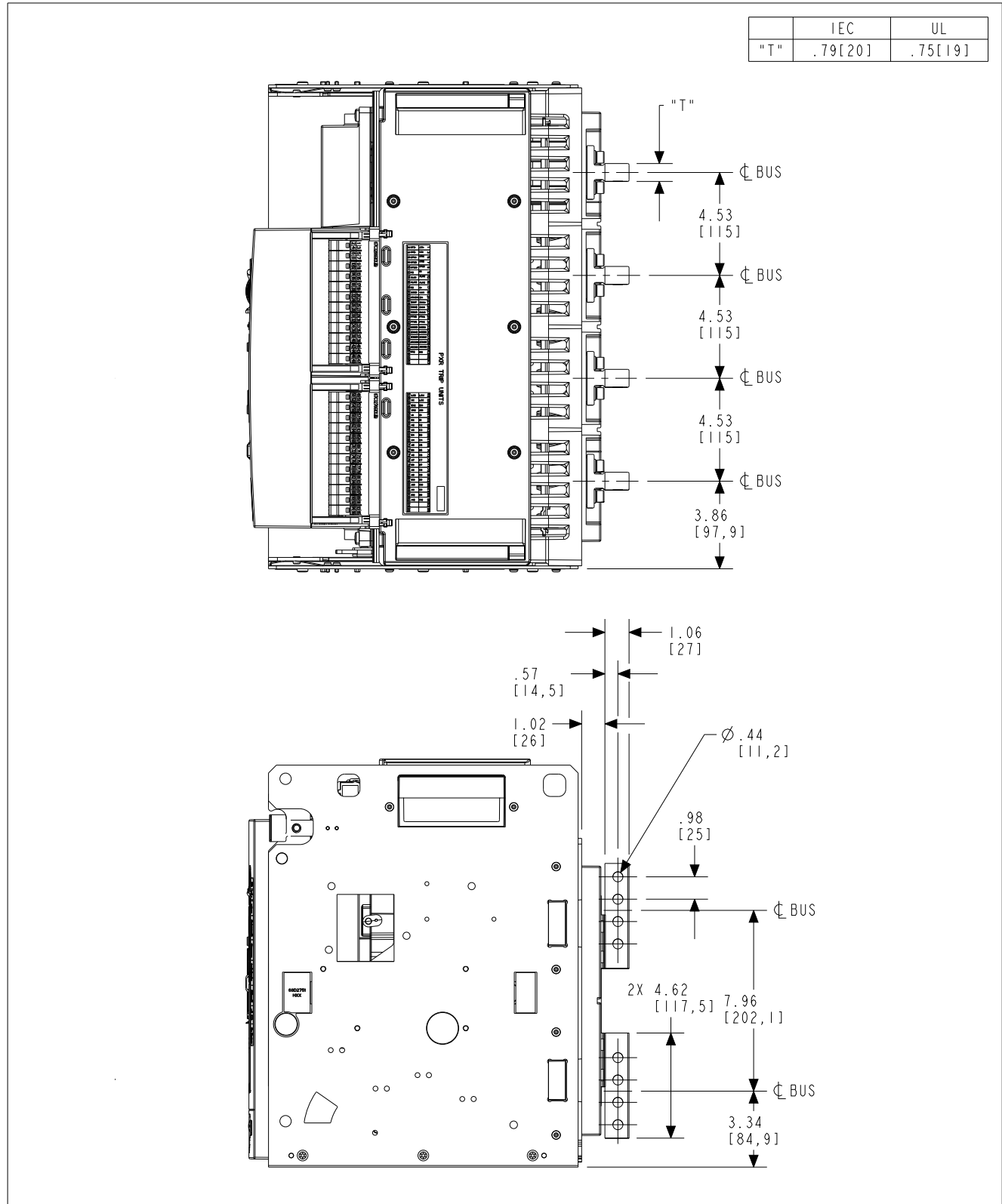
Figure 48. Four-pole drawout cassette - top/side views with offset four-hole vertical bus adapters in inches (mm).
