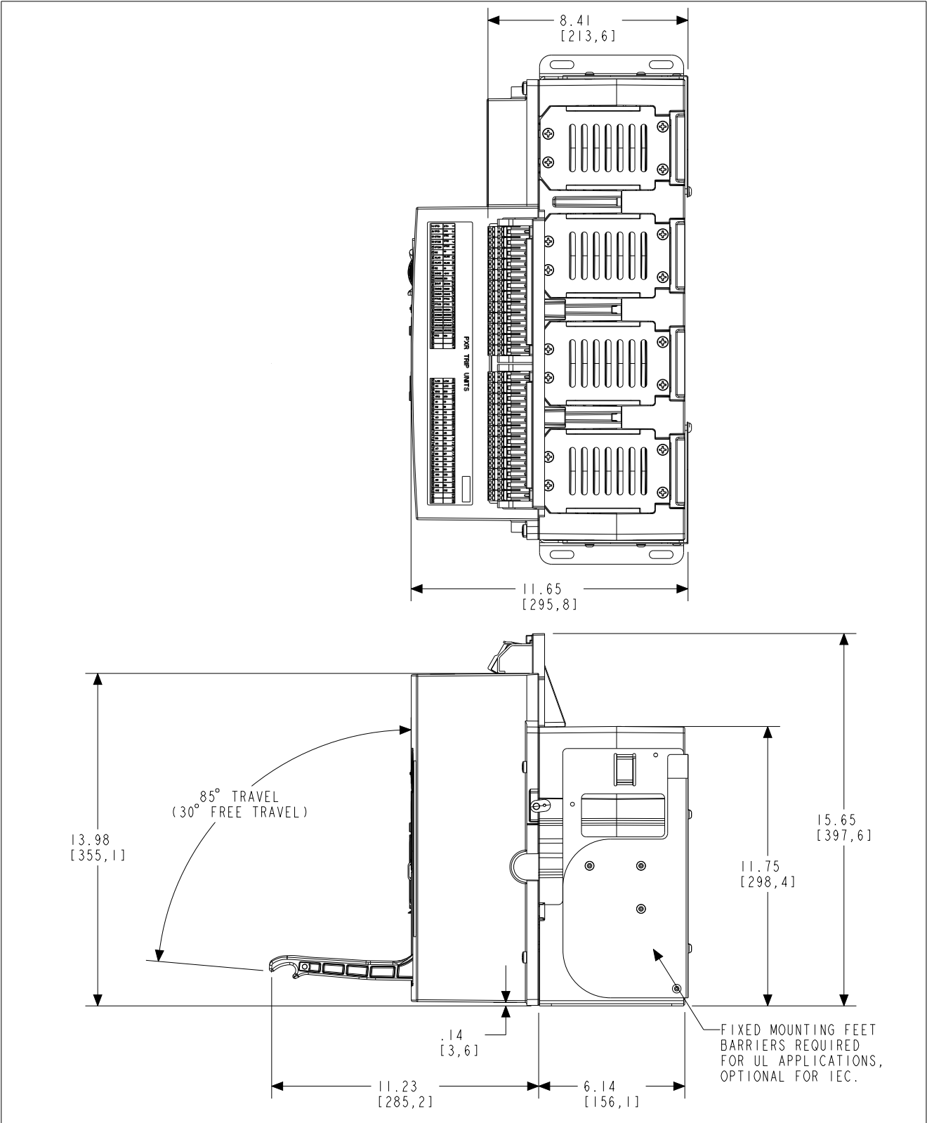
Figure 60. Four-pole fixed breaker - top/side views in inches (mm).
