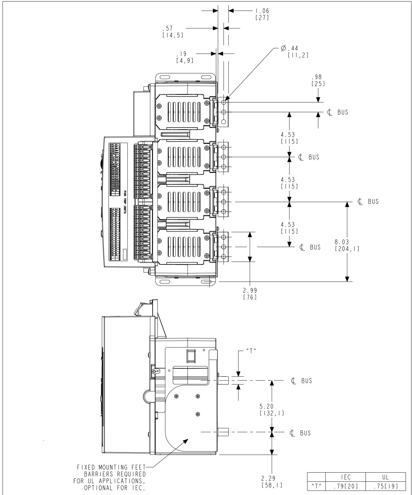
Figure 61. Four-pole fixed breaker - top/side views with centered three-hole horizontal bus adapter in inches (mm).
