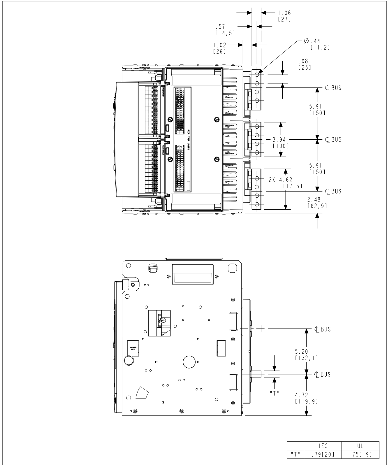
Figure 38. Three-pole drawout cassette - top/side views with offset four-hole horizontal bus adapters in inches (mm).
