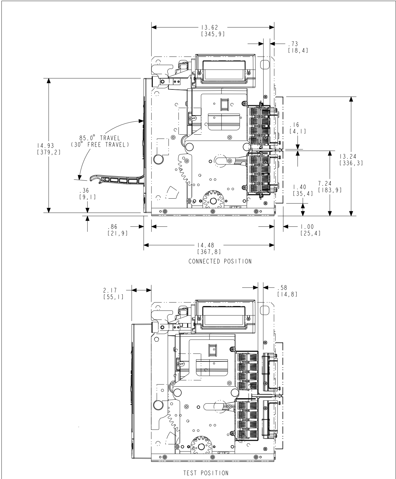
Figure 43. Four-pole drawout cassette - side views CONNECTED and TEST positions in inches (mm).
