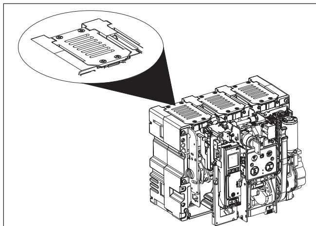
Figure 70. Step 3.
