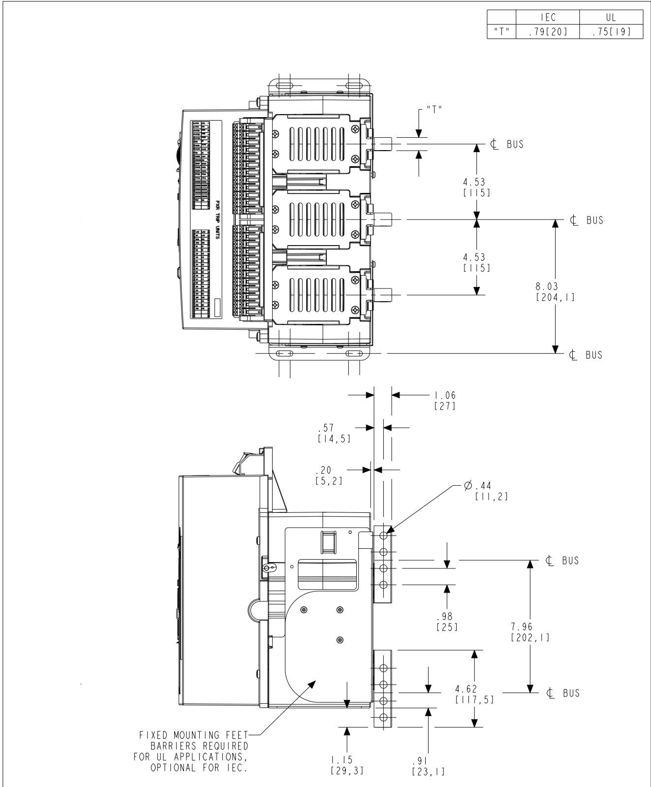
Figure 56. Three-pole fixed breaker - top/side views with offset four-hole vertical bus adapter in inches (mm).
