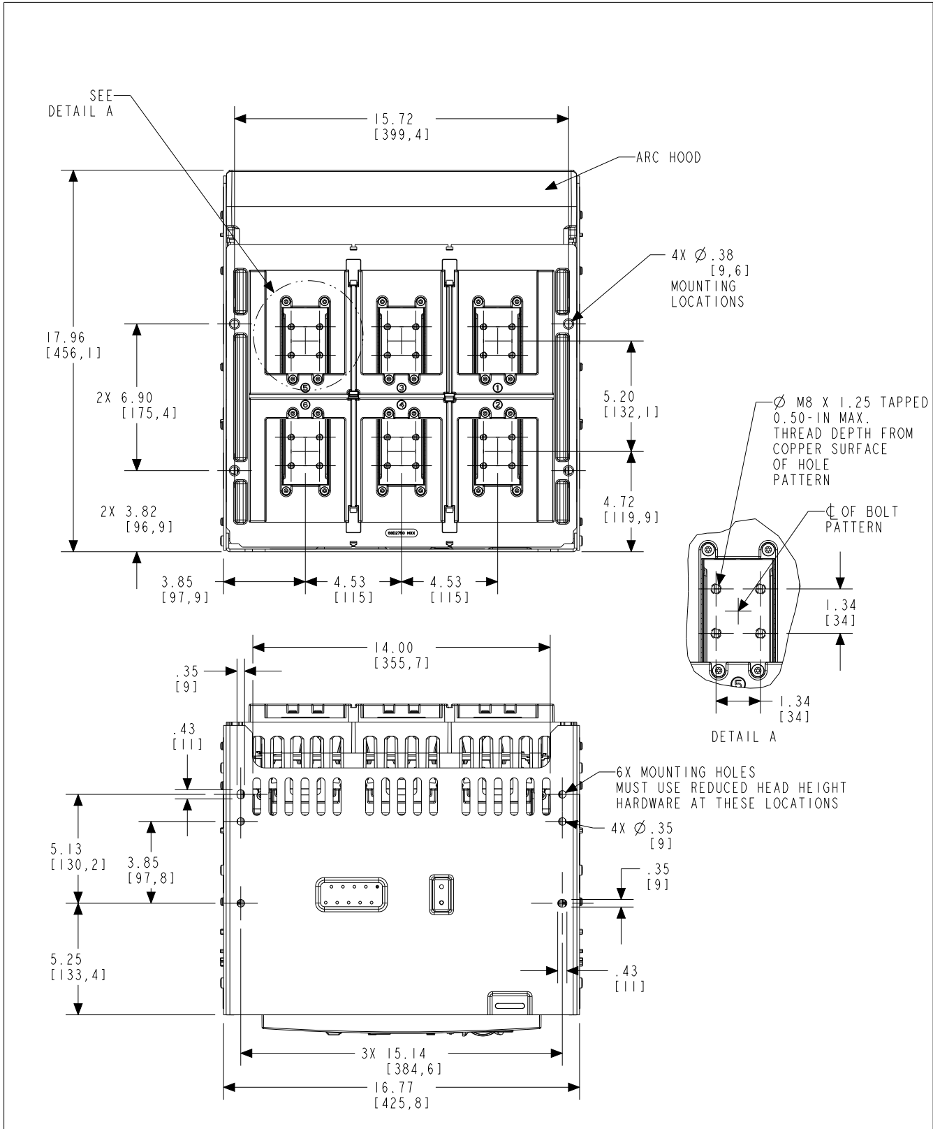
Figure 33. Three-pole drawout cassette - rear/bottom views in inches (mm).
