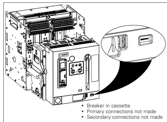
Figure 16. WITHDRAWN position.
