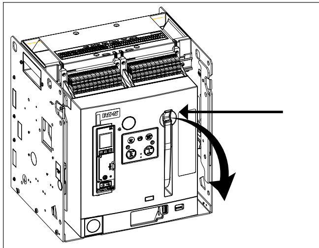
Figure 24. Step 1.
