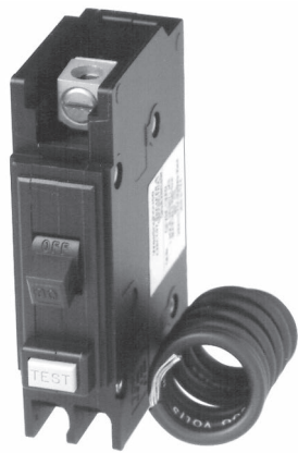
QUICKLAG Type QCGFT Single-Pole Ground Fault Circuit Breaker
