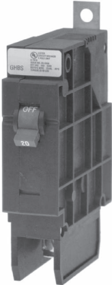
GHBS and GHQRSP
