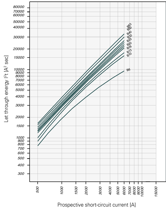
Let-through Energy HN, Characteristic B, 1-pole
